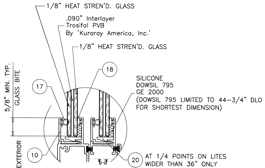
GLAZING DETAIL 5/16" OVERALL LAM. GLASS
